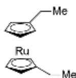
Figure 3. Molecular formula of bis(ethylcyclopentadienyl)ruthenium(II) (EtCp) 2 Ru.
