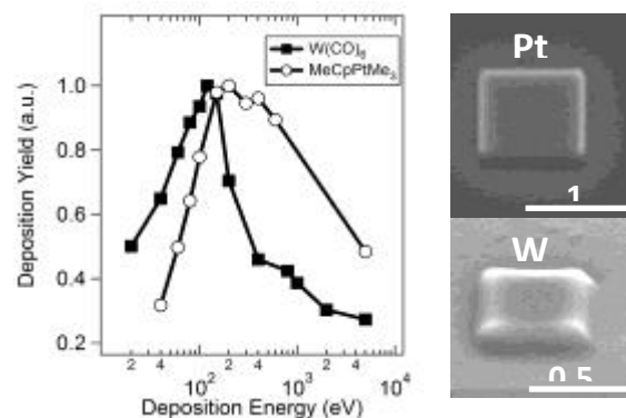
Fig.1 (left) Deposition Yield measured by AFM and (right) SEM images of Pt and W squares deposited at 80 eV.
