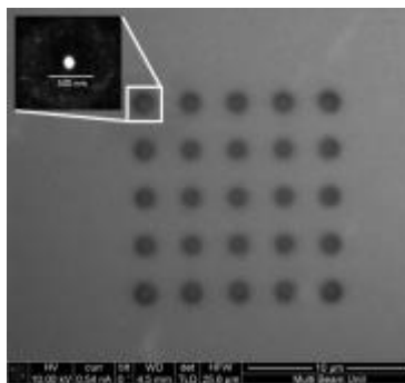
Figure 3. A 5x5 array of EBID pillars deposited in a single 5 s exposure. The inset shows a zoomed-in image of one of the pillars, with a diameter of 90 nm.
