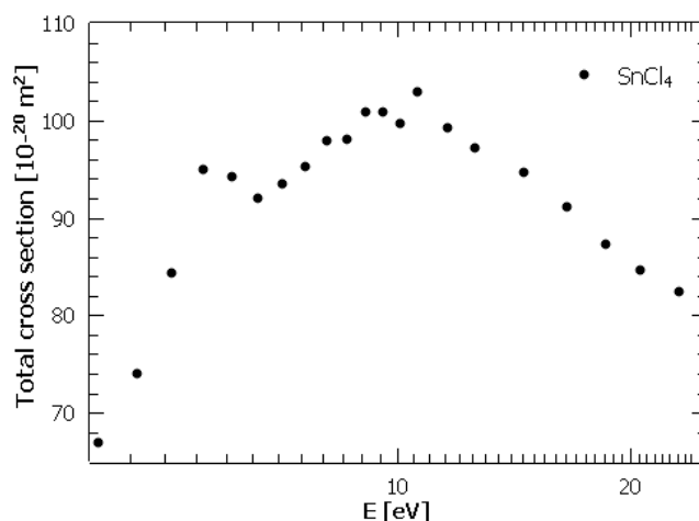
Fig. 1. Preliminary results of experimental TCS for electron scattering from SnCl 4 .
