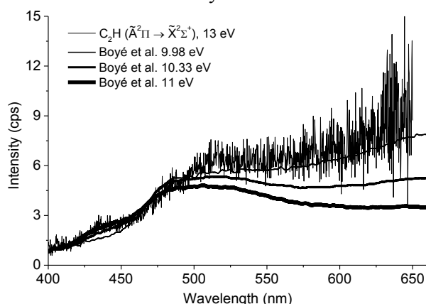
Fig. 1. Ethynyl radical spectrum.
