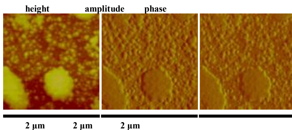
Figure 1. AFM images of [Cu(II)(-)-chxn(3,5- 1 Buba)(5-nba)] (spin coating 100 rpm, 5s), after heating, magn. 2 \mu\text{m} .
