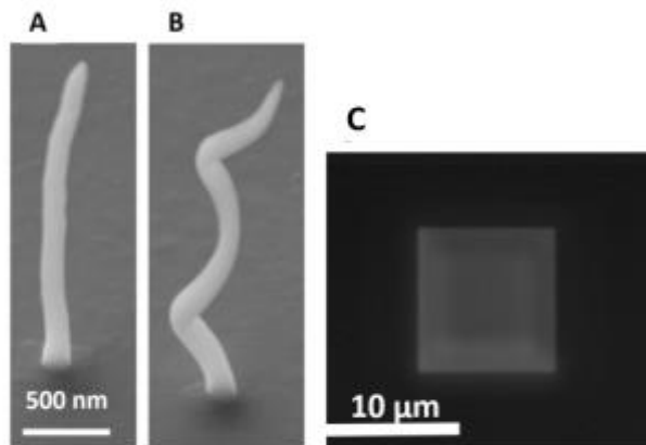
Figure 4 A,B) Scanning electron micrograph of nanostructures fabricated with the new copper precursor. C) Scanning electron micrograph of a square deposit on a transparent substrate used for transmission/reflection measurement to determine the permittivity.
