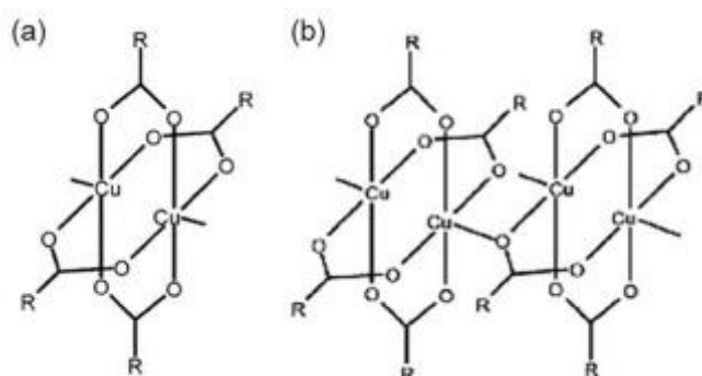
Figure 1 The examples of copper(II) carboxylate compounds structures a) a “paddle wheel” dimer b) a polymeric chain.
