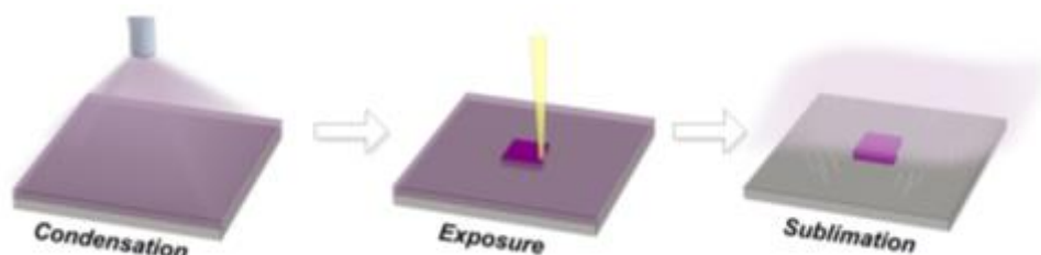
Figure 1. OIR process: a vapour of an organic compound is first condensed onto the cooled sample to form a uniform layer. Its interaction with the e-beam locally modifies its chemical composition resulting in a non-volatile product. When the sample is heated to room temperature the unexposed OIR sublimates while the exposed patterns are stable, enabling ambient downstream processing.
