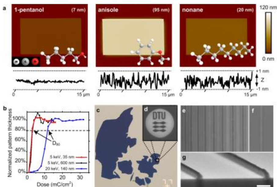
Figure 2. AFM images of 20 x 12 \mu\text{m}^2 rectangles patterned in OIR thin-films and representative scan-lines across the rectangle surface (a). b, contrast curves for nonane ice at 5 and 20 keV. The critical dose at 5 keV is unchanged even with a 20-fold time increase in thickness. c-d, large area map of Denmark made by exposed nonane ice (dark blue areas). The total exposure time was 75 min. The optical image (c) covers an area of 0.4 x 0.5 mm 2 . e, SEM image of 100-nm-wide lines patterned in nonane ice. f, 60-nm-wide line patterned in anisole ice. g, Tilted SEM view of patterned OIR lines reaching the edge of a 1 x 1 cm 2 chip. The OIR layer is uniform on the entire sample surface, up to the very edge. Scale bar is 200 nm.
