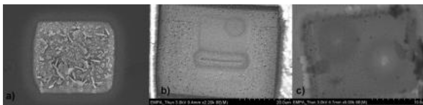
Figure 2: Top view SEM images of FEBID deposits obtained at 20 keV and 0.9 nA on native oxide silicon substrates. a) 10\ \mu\text{m} \times 10\ \mu\text{m} rectangle by [\text{Ag}(\text{O}_2\text{CC}_2\text{F}_5)] (1) showing silver platelets. b) line and dot deposit by [\text{Ag}(\text{O}_2\text{CC}_4\text{F}_9)] (2), note the halo around these structures, c) dot deposits by [\text{Ag}(\text{O}_2\text{CCHEt}_2)] (3) containing no silver.
