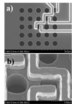
Figure 4. a) Top view SEM micrograph of the 3 micro blankers, and b) the rotated, tilted and zoomed-in view of one of the deflectors (b).
