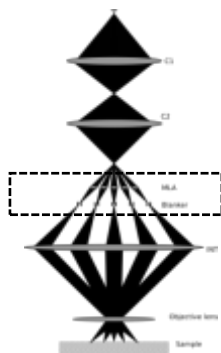
Figure 1. The design of a multi-beam SEM. The micro lens array (MLA) and blanker are indicated.
