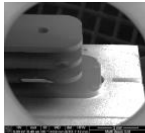
Figure 2. A SEM micrograph is shown of the stack of electrodes forming the MBU.
