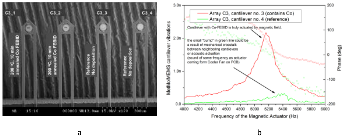
Fig.1. The fabricated cantilevers with Co/C FEBID pattern (a) SEM image, (b) deflection comparison: with and without Co/C pattern.
