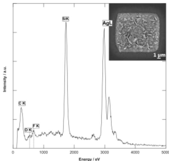
Figure 1 – EDX spectrum of a silver rectangle written by a focused electron beam (20 keV, 0.9 nA) on a native SiO 2 /Si substrate. The metal content was determined to be 76 % after subtraction of the substrate signal. The inset displays a SEM image of the deposit.
