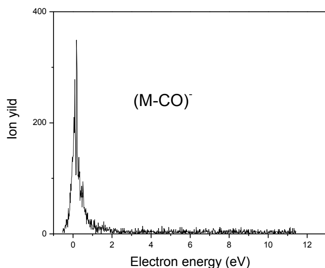
Fig.1. Ion yield of (M-(CO))^- , produced from electron impact on gaseous cyclopentadienylmanganese(I) tricarbonyl.
