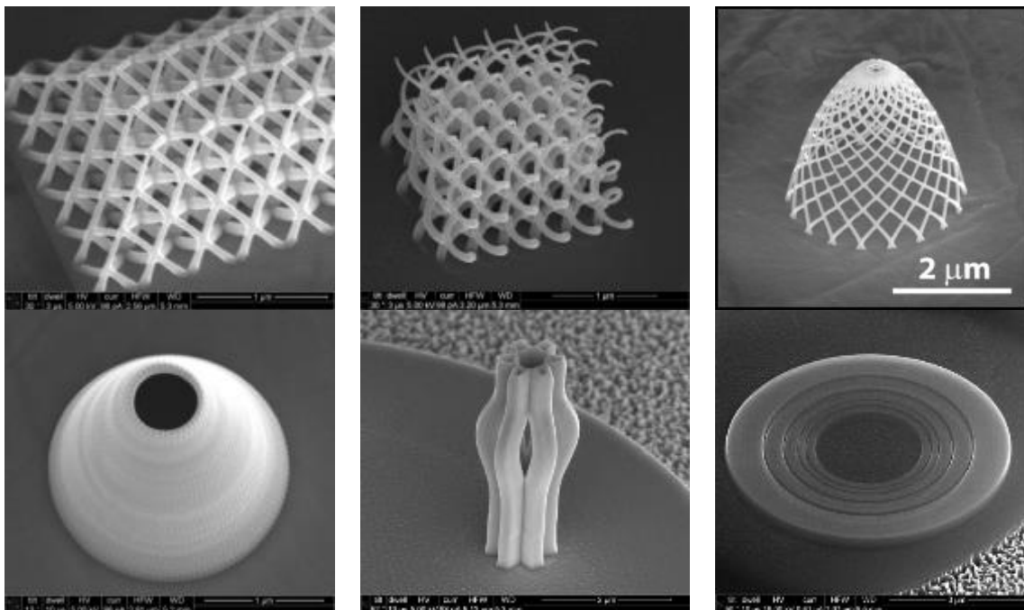
Figure 1. Examples of 3D structures grown by EBID using MeCpPtMe 3 as a precursor.
